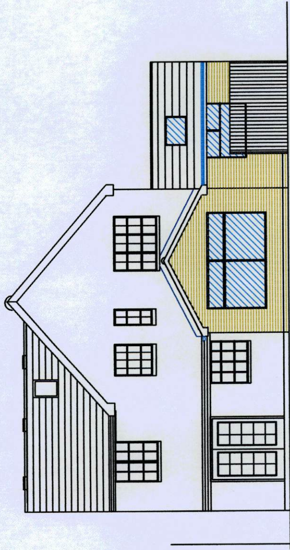
Rear Elevation
